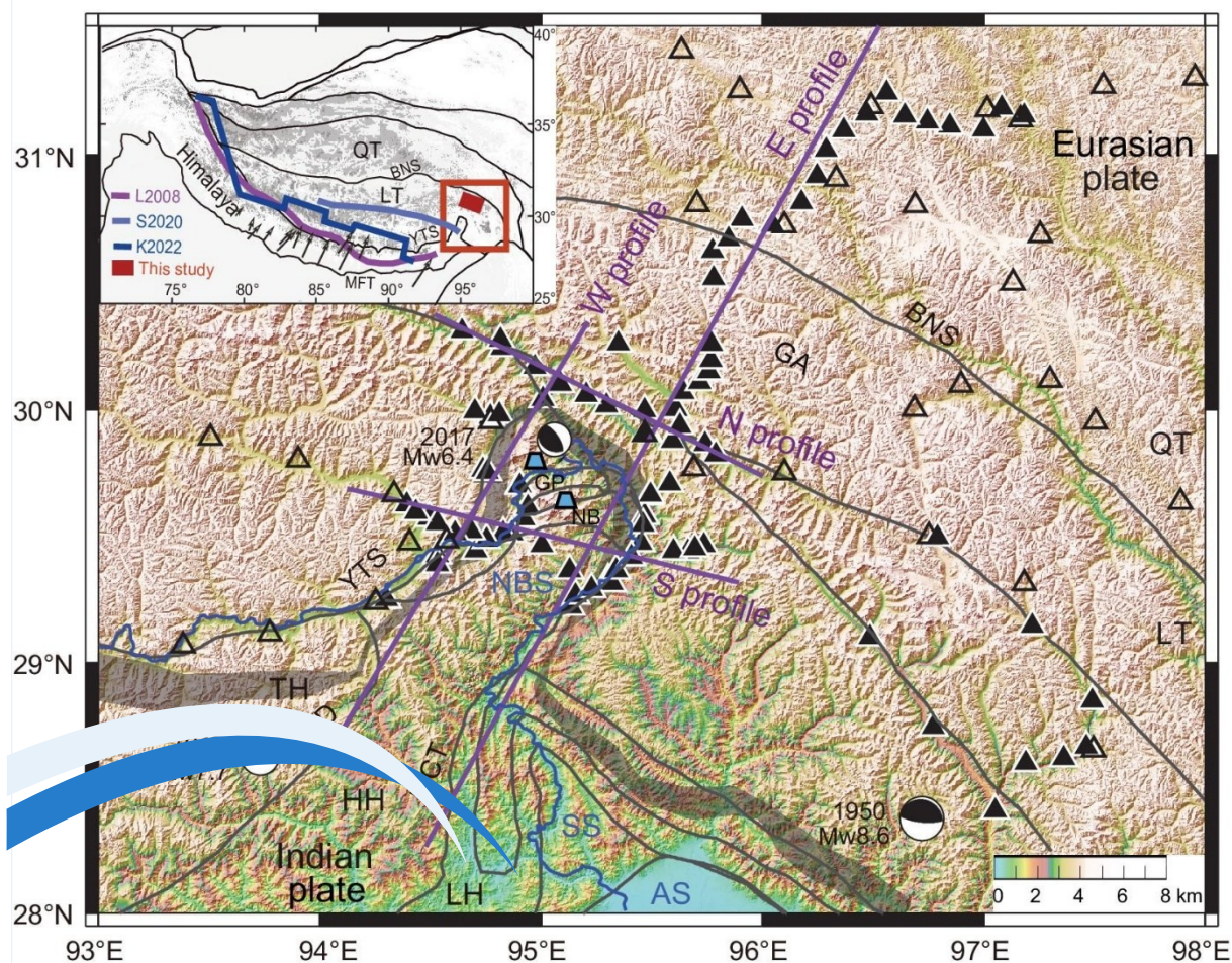
Fig. 2. Tectonic map with seismic stations. From Bai Ling's paper.
